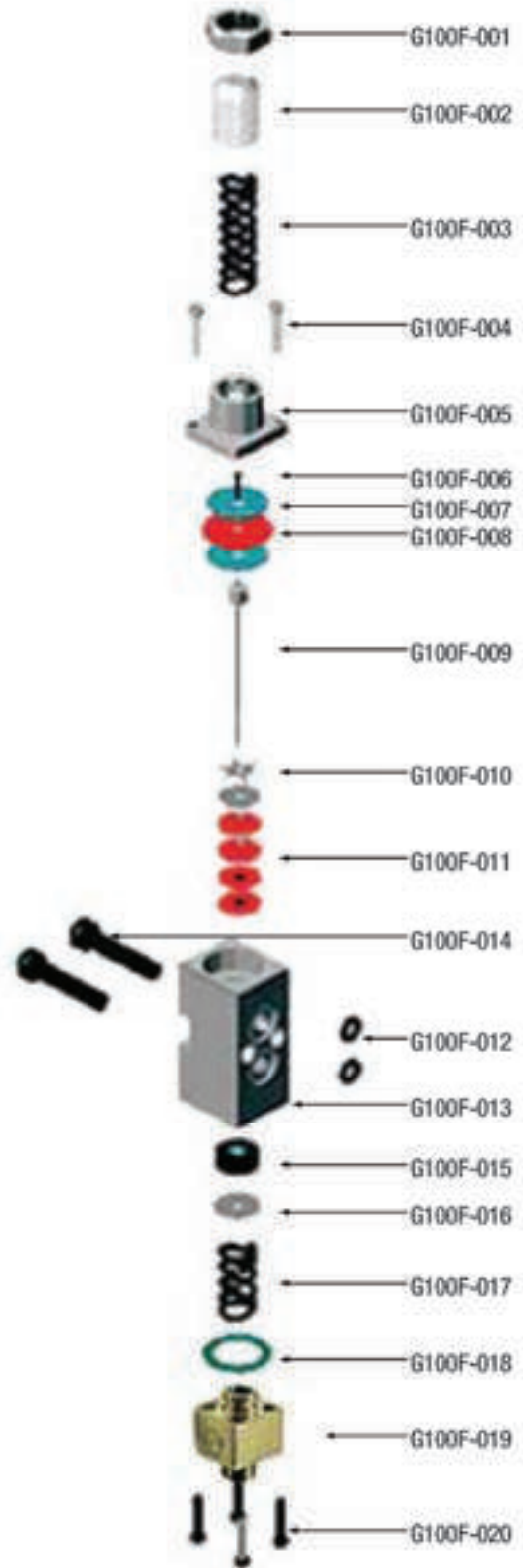
G100F-017 Spring 27/64 x 33/64 $1.10
